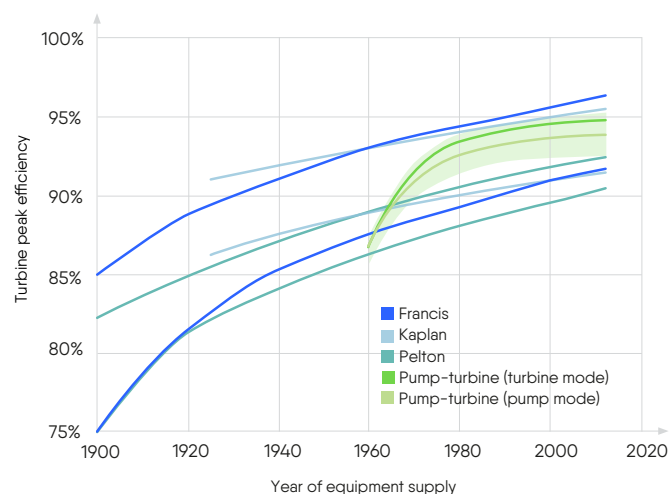
Figure 1: Efficiency development of turbines 2
